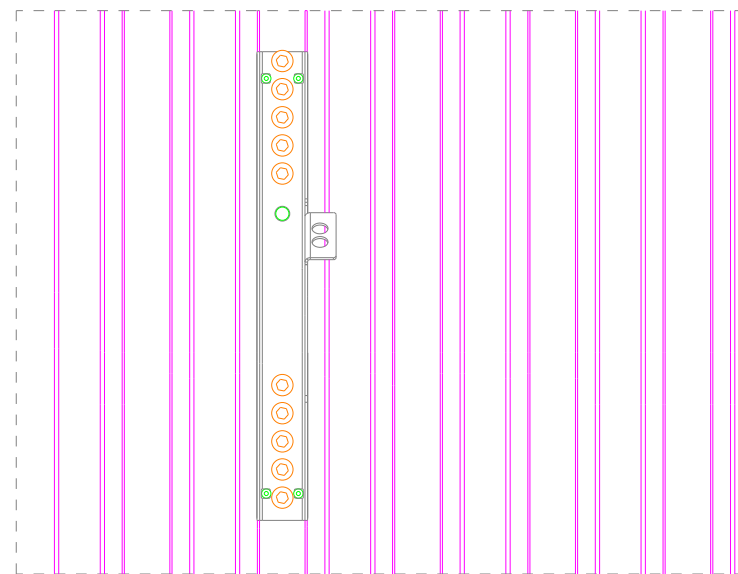
Bracket mounted on sheet metal
